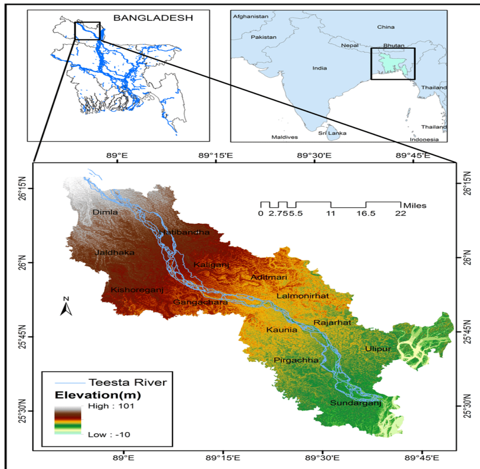
Fig. 1. Teesta Watershed [19]
