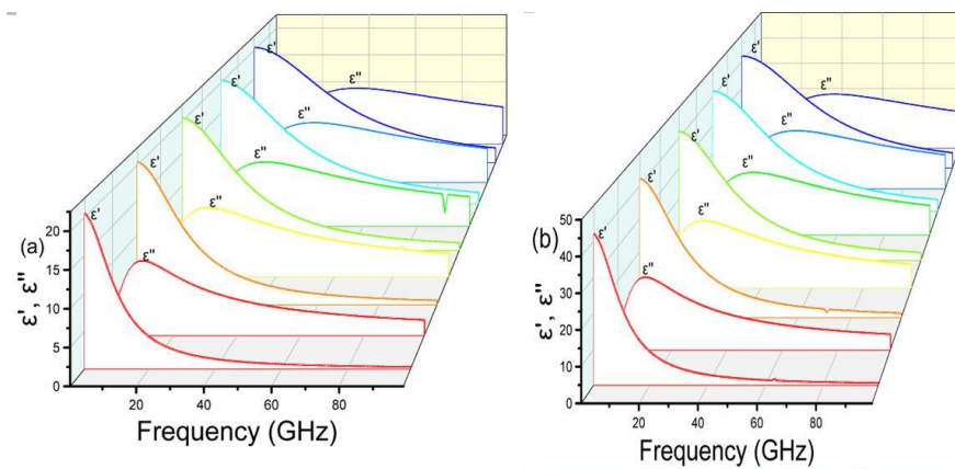
Fig. 7. Frequency dependency of the dielectric constant ( \epsilon' ) and loss factor ( \epsilon'' ) of (a) Graphene and (b) G4/T10/PVDF
