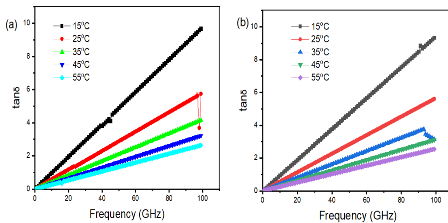
Fig. 5. The loss tangent against the frequency (a) Graphene and (b) G4/T10/PVDF at different temperatures
