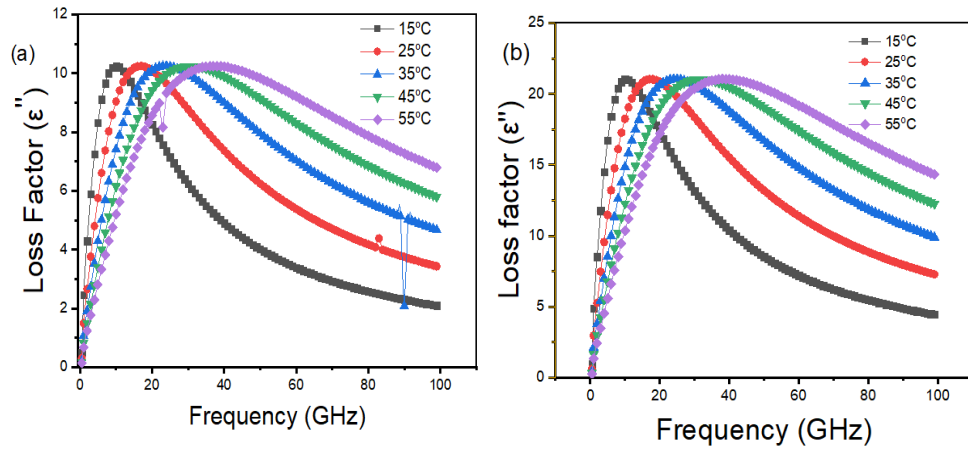
Fig. 3. Frequency dependence of loss factor ( \epsilon'' ) of (a) Graphene and (b) G4/T10/PVDF at indicated temperatures
