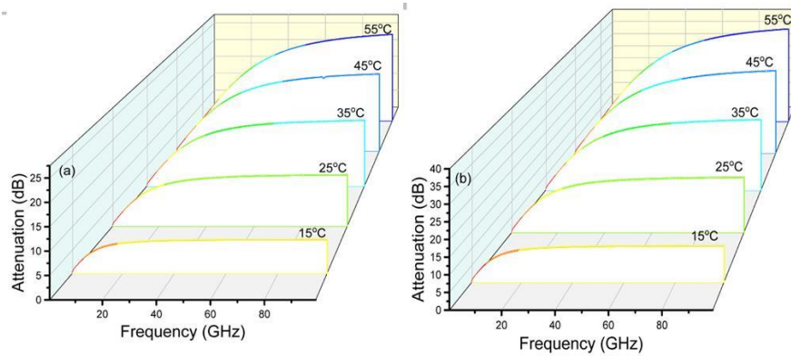
Fig. 6. Frequency dependency of the attenuation of (a) Graphene and (b) G4/T10/PVDF at the indicated temperatures
