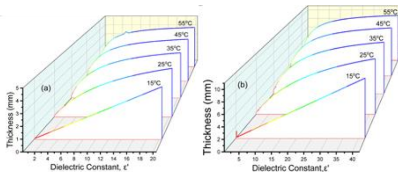
Fig. 8. The behaviour of Thickness against the dielectric constant at different temperatures (a) Graphene (b) G4/T10/PVDF
