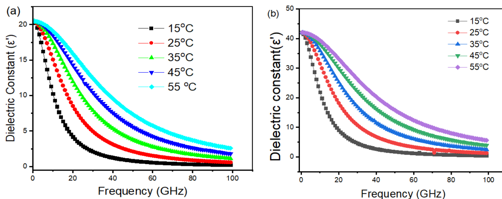
Fig. 2. Frequency dependence of dielectric constant ( \varepsilon' ) of (a) Graphene and (b) G4/T10/PVDF at indicated temperatures
