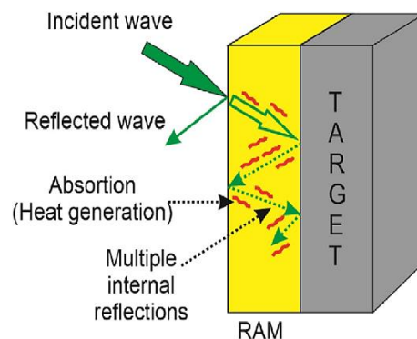
Fig. 1. Schematic diagram of absorption and multiple reflections of RAMs as attenuation mechanisms [23-24]
