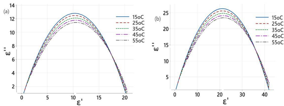
Fig. 4. The plots of \epsilon''(\omega) against \epsilon'(\omega) in Cartesian coordinates for (a) Graphene (b) G4/T10/PVDF
