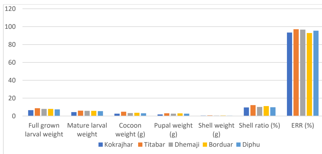
Fig. 1. Larval weight and cocoon characters of different eco-races of eri silkworm
